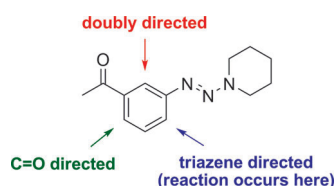
Figure 1. Selectivity in the presence of a second directing group.
